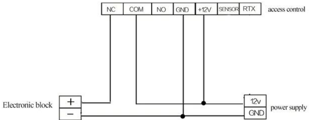
Wiring diagram
