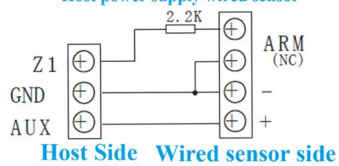
Host power supply wired sensor
