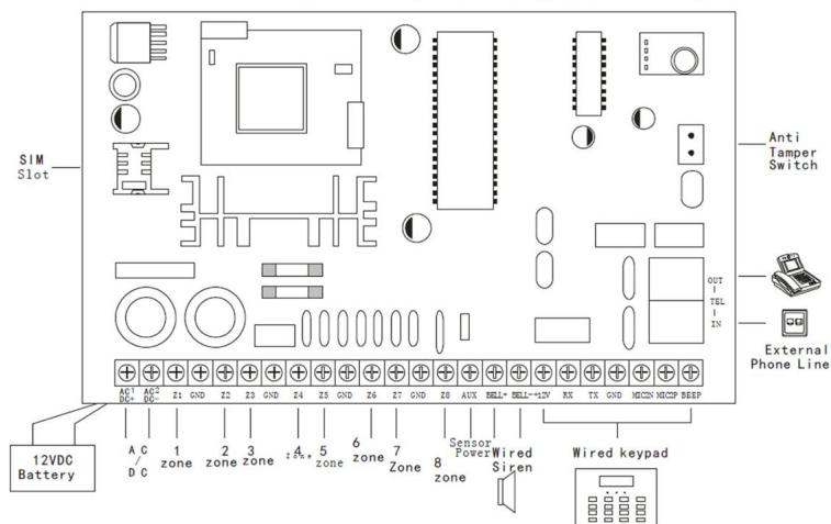
Host power supply wired sensor
