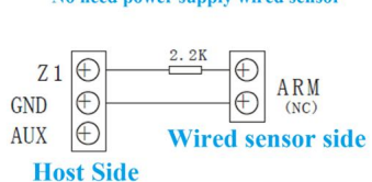
No need power supply wired sensor
