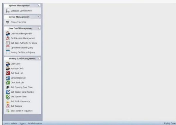
Software interface
