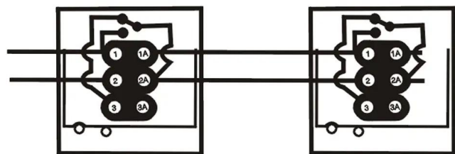
NC circuit wiring way
