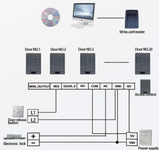
Wiring diagram
