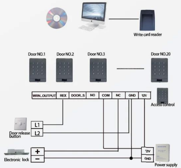
Wiring diagram
