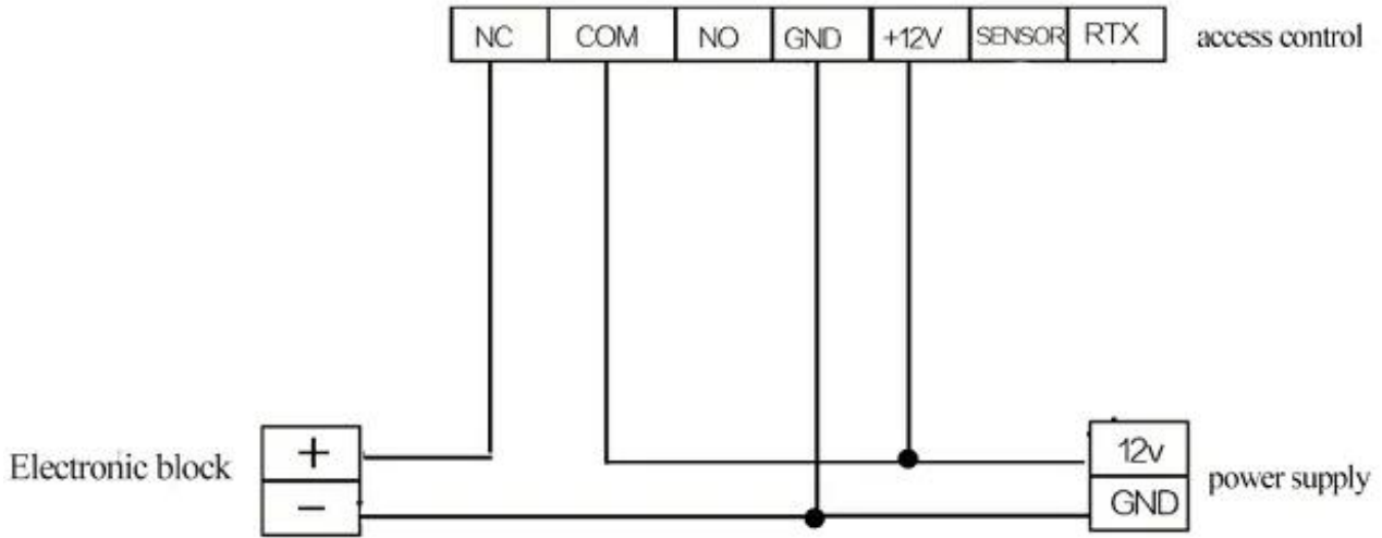
Wiring diagram
