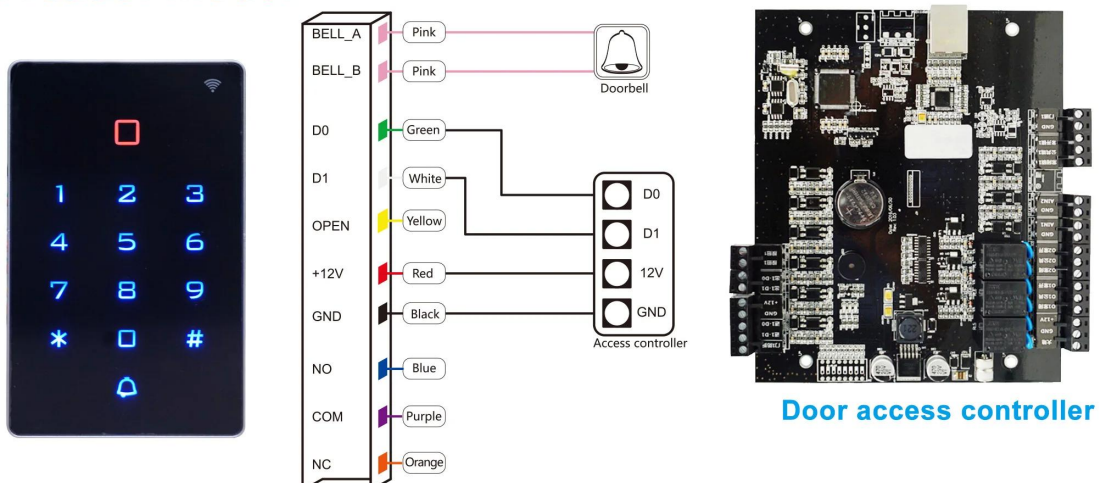
Connect with access controller to working as a reader
