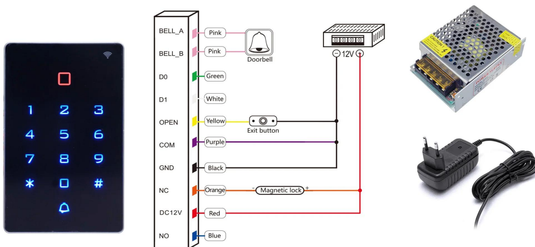
B: Use normal DC12V power supply
