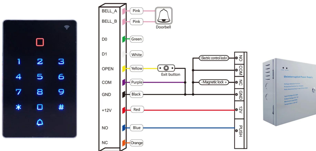
A: Use access control switch power supply
