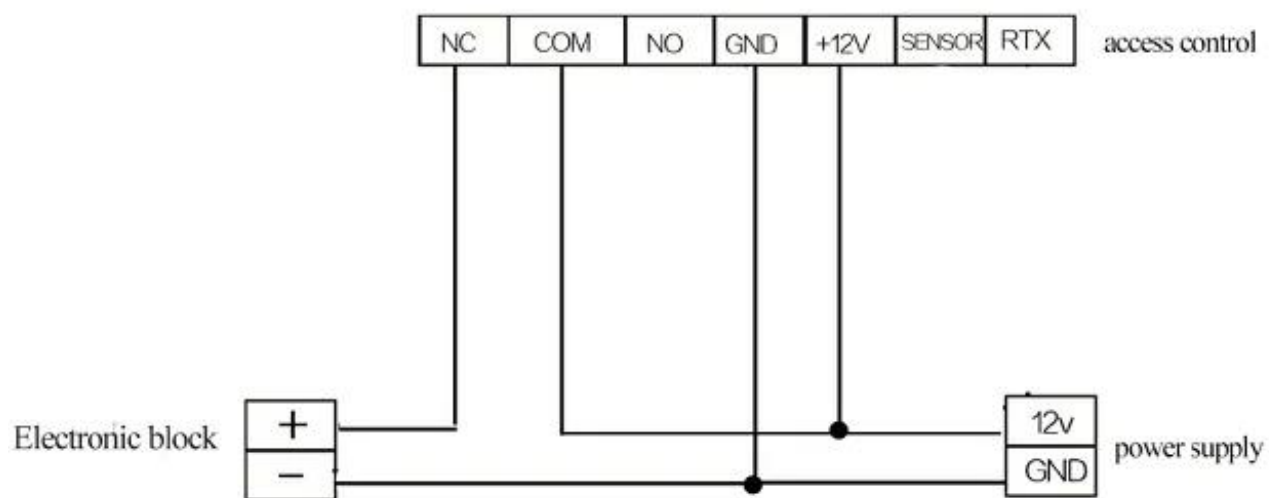
Wiring diagram
